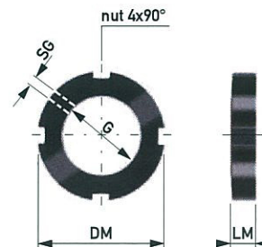
Draw-off nut with anti rotation nut similar to DIN 1804 with thread for locking pin
