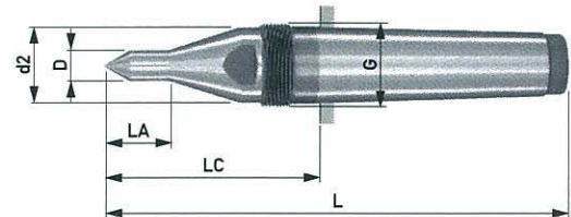
Form 257 slim design 60°/35°
